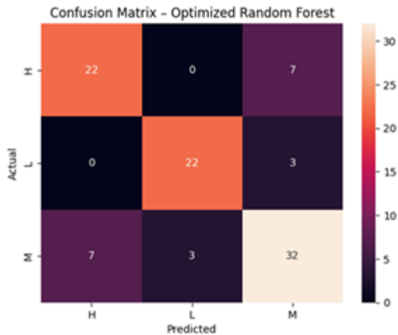
Figure 2. Confusion Matrix - Optimized Random Forest
