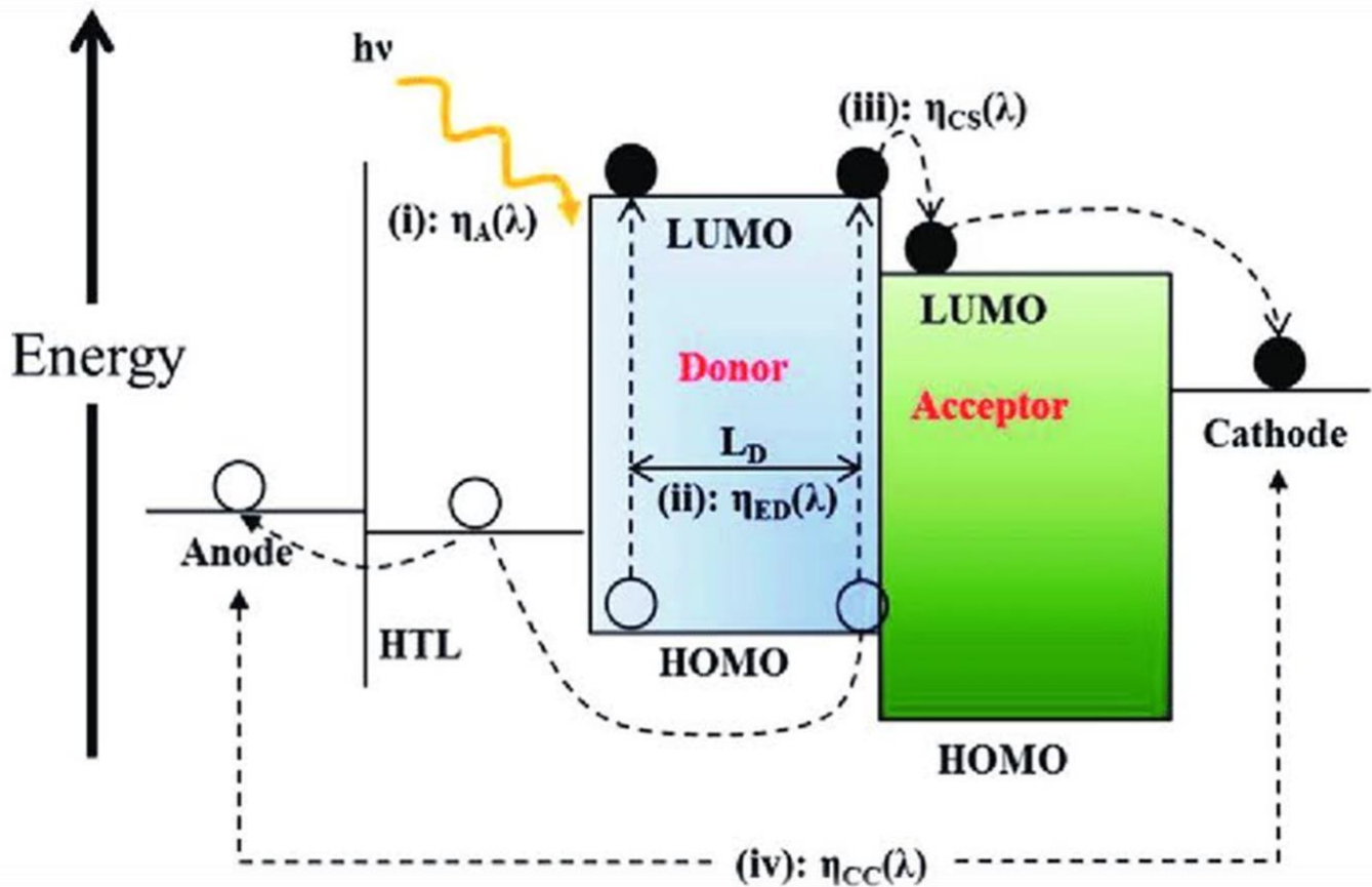
Figure 3: Organic Solar cell
