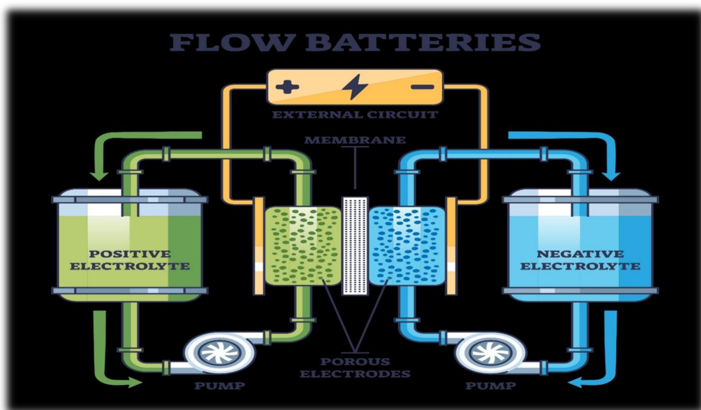
Figure 4: flow battery
