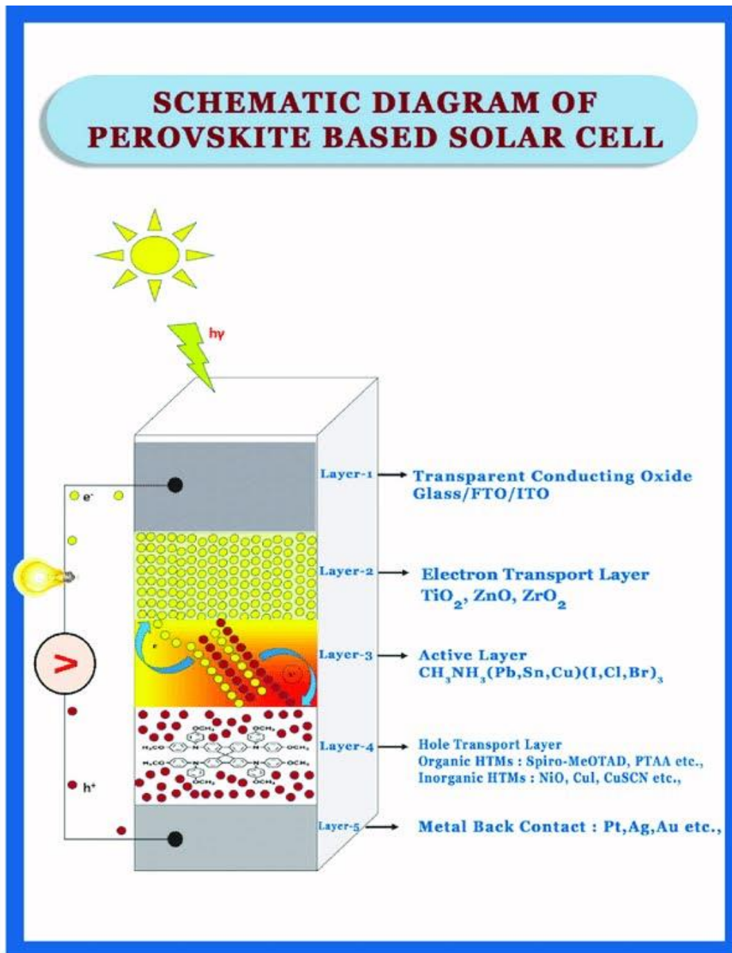
Figure 2: Perovskite Solar Cell
