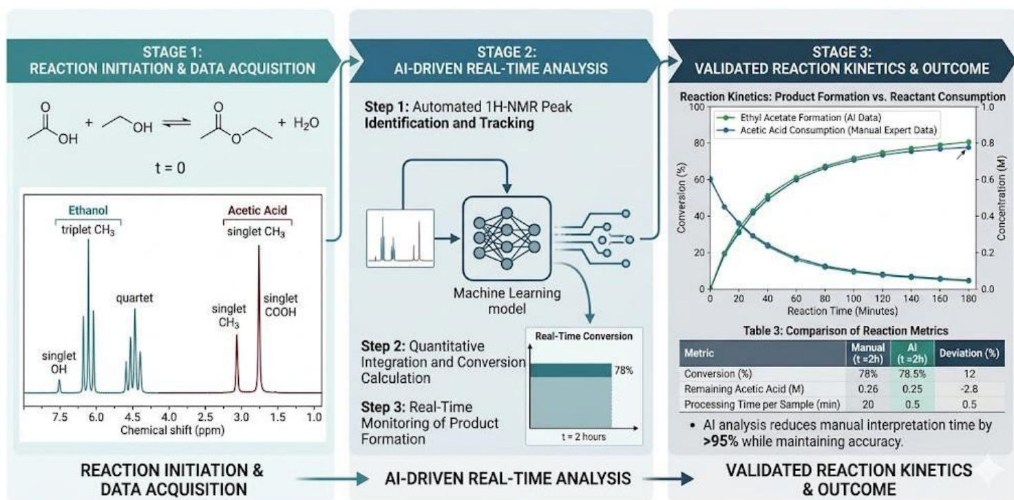
FIGURE 3: CASE STUDY: AI-DRIVEN REACTION MONITORING OF ETHYL ACETATE SYNTHESIS
