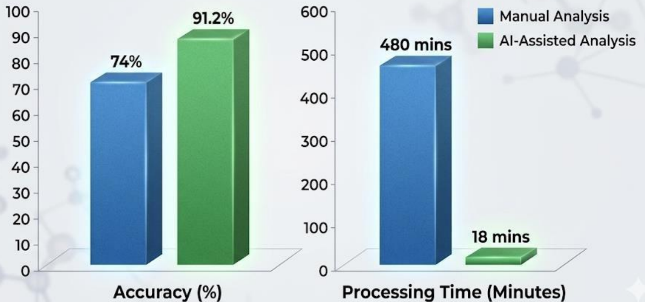
Figure 1: Comparison of Analytical Performance: Manual vs. AI-Assisted Methods
