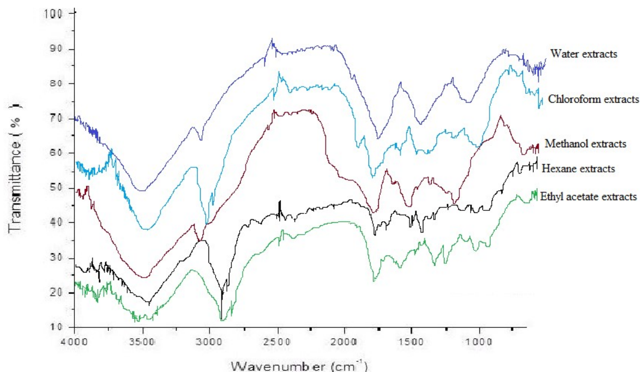
Figure 1; FT-IR spectra of S. didymobotrya leaves extracts
