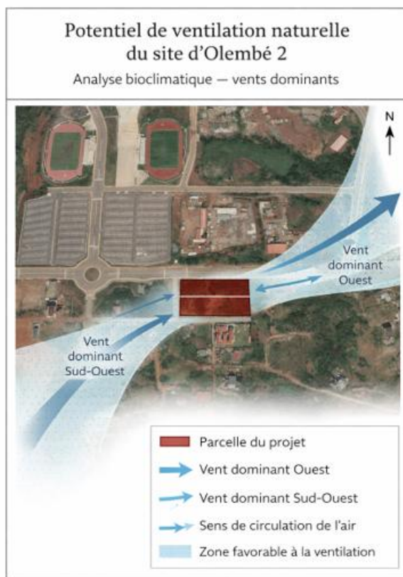
Figure 3. Natural-ventilation potential of the Olembé 2 site, showing the project plot's exposure to the dominant west and south-west winds. (Source: Tene Fosso, 2026.)
