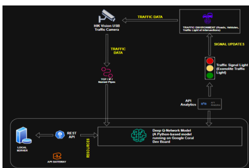
Figure 2: System Architecture for Real-Time Traffic Signal Optimisation System.
