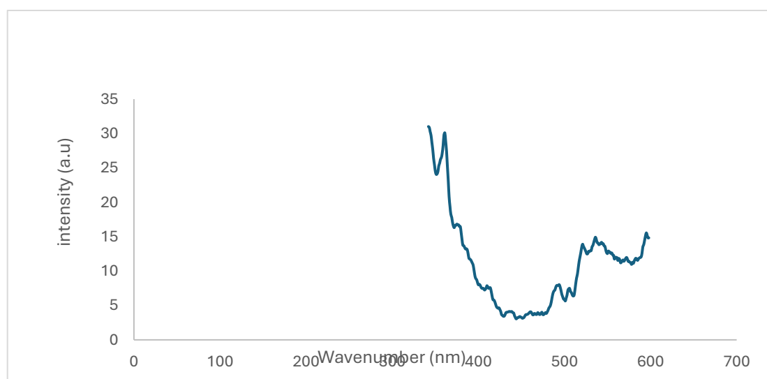
Fig.3 Photoluminus spectra of CdS/ZnS/PVA nanocomposites
