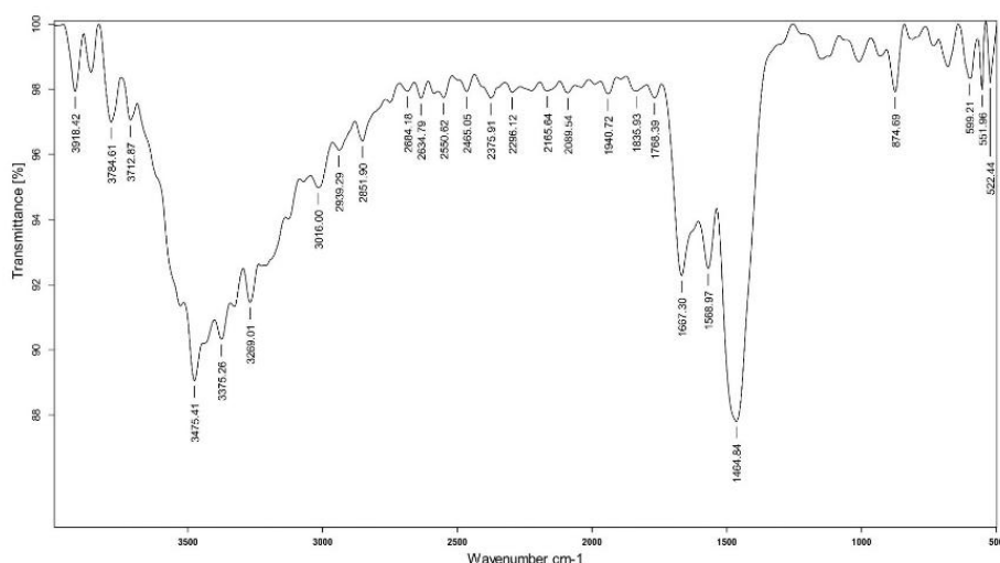
Fig.2 FT-IR Spectra of CdS/ZnS/PVA nanocomposites
