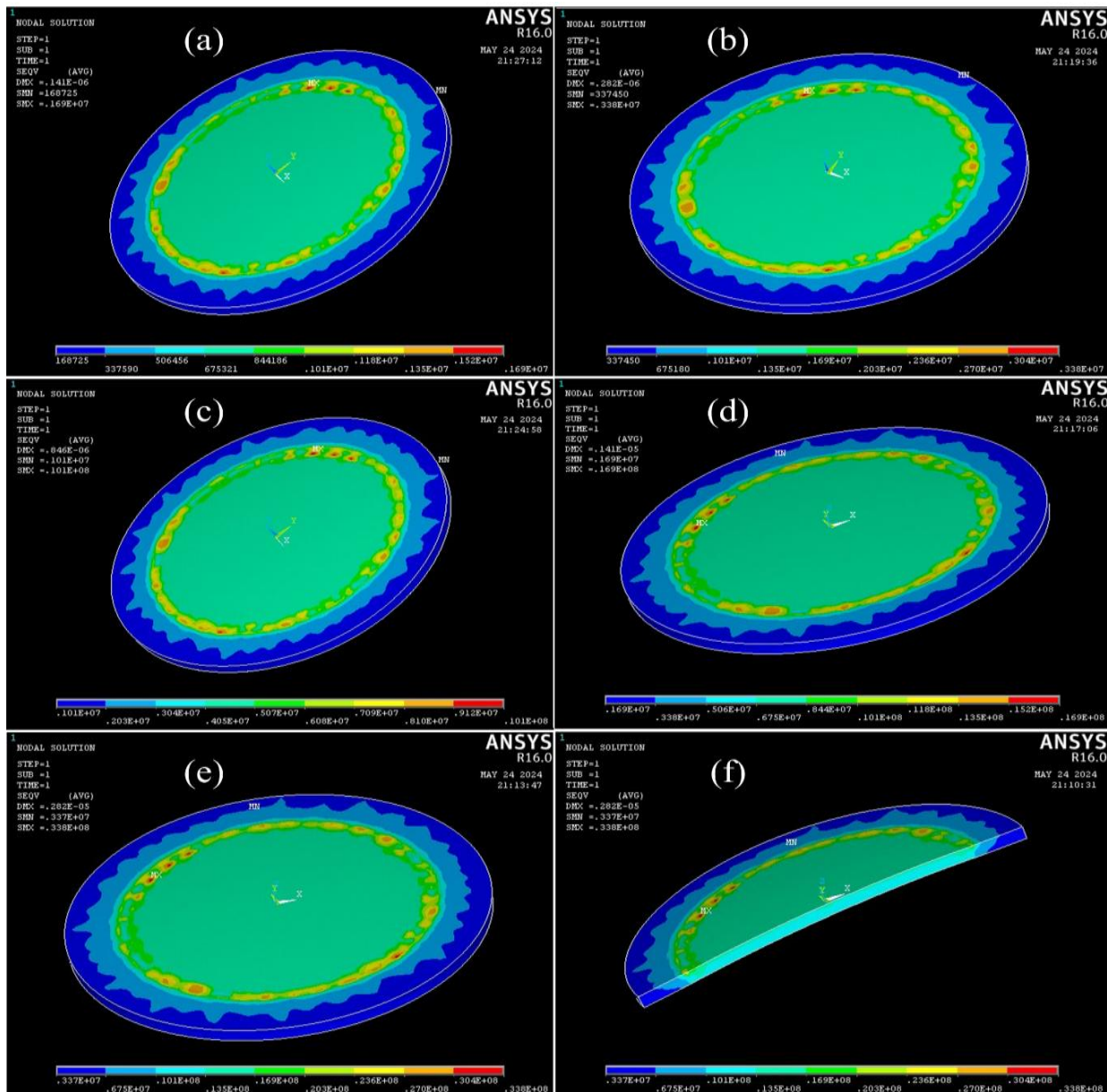
Figure. 2. Stress distribution with variation pressure applied in the designed assembly device
