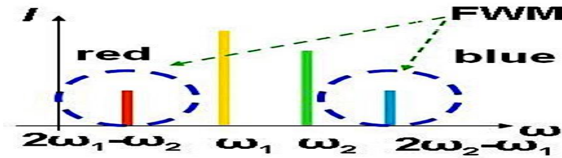
Fig. 3 SOA FWM mechanism (44)
