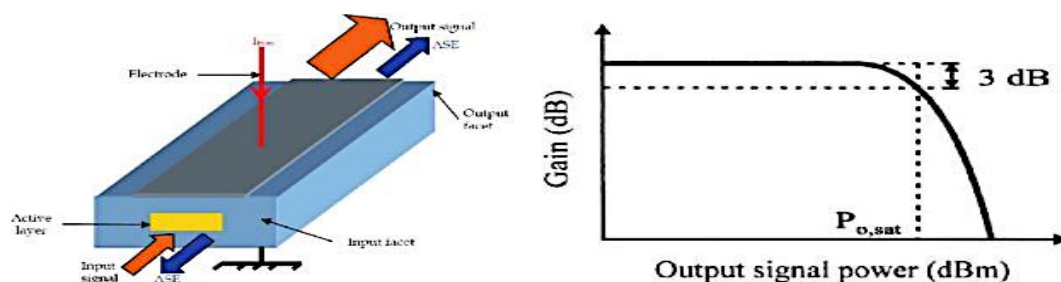
Fig. 1 SOA gain mechanism [62]
