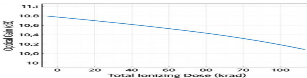
Fig. 7 Optical gain stability of a radiation-hardened SOA-PIC under ionizing radiation up to \sim 100 krad, showing < 1 dB degradation—demonstrating robustness for space applications [100]
