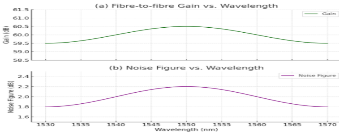
Fig. 23 Measured performance of the Raman-assisted SOA reported in [170], showing (a) flat fibre-to-fibre gain of ~60 dB over 1530–1570 nm and (b) noise figure consistently around 2 dB across the band [170].
