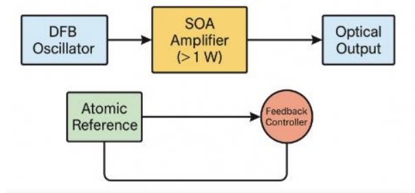
Fig. 25 Frequency-stabilized DFB-SOA laser system integrating a DFB oscillator, >1 W SOA amplifier, and atomic-reference feedback control for sub-MHz linewidth stability in portable cold-atom applications [175].
