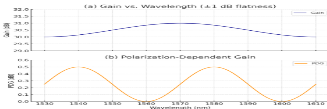
Fig. 24 Measured performance of the QD-SOA, showing (a) >30 dB gain with \pm 1 dB flatness over 1530–1610 nm and (b) polarization-dependent gain <0.5 dB across the full bandwidth [172].
