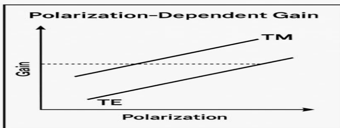
Fig. 15 Polarization-dependent gain in a traveling-wave semiconductor laser amplifier (TW-SLA), illustrating higher gain for TM-polarized light compared to TE-polarized light. The gain disparity highlights the inherent polarization sensitivity of early SOA designs [117].
