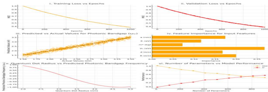
Fig. 20 Machine learning optimization results showing (i-ii) convergence, (iii) prediction accuracy, and (iv-v) parameter sensitivity for quantum dot superlattice photonic properties. [146]
