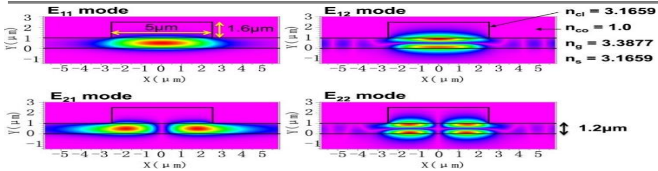
Fig. 18 Simulated mode profiles in a multimode SOA showing efficient gain overlap via mode-division multiplexing, enabling 87% gain enhancement [141].
