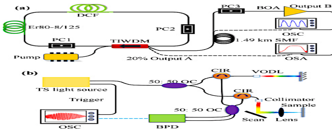
Fig. 16 experimental set-up used to incorporate a BOA (booster SOA) [123]
