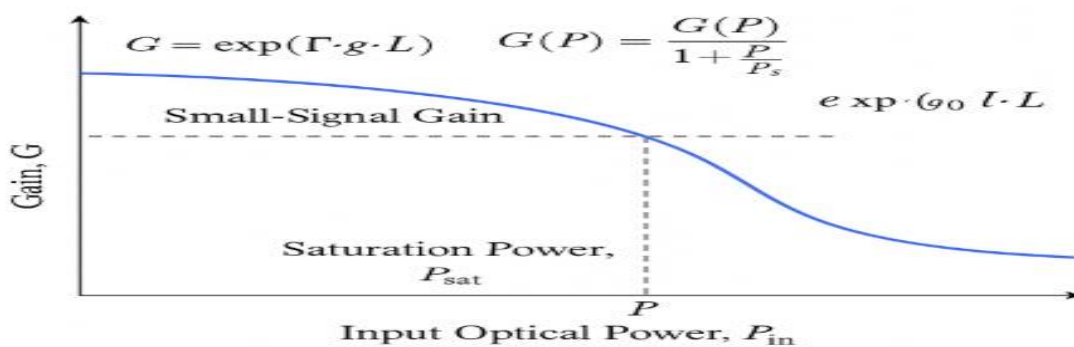
Fig. 2 Gain versus input optical power in a semiconductor optical amplifier (SOA), illustrating small-signal gain, gain saturation, and the typical exponential gain behaviour [42].
