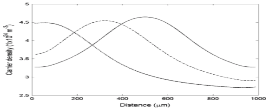
Fig. 17 Simulated carrier density spatial distributions for TM polarised signal input powers of -40 dBm (solid line), -10 dBm (dashed line) and 0 dBm (dotted line). The bias current and signal wavelength are 200 mA and 1550 nm, respectively. [132]
