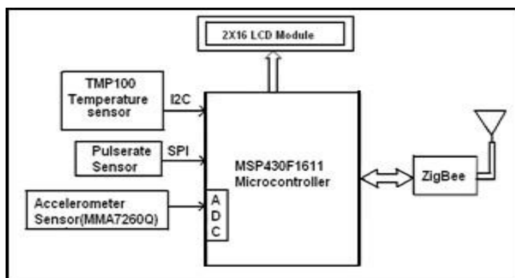
Figure 2. Block diagram of the design
