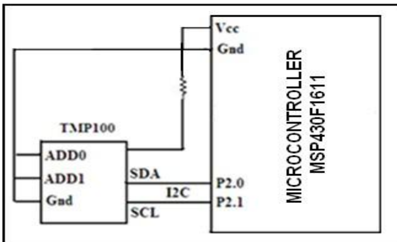
Figure 4. Interfacing of Digital temperature sensor TMP100
