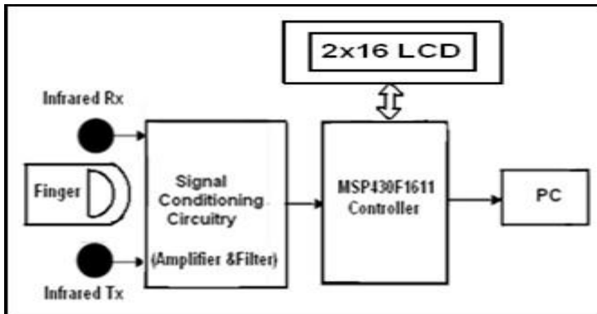
Figure 5. Block diagram of Pulse rate measurement
