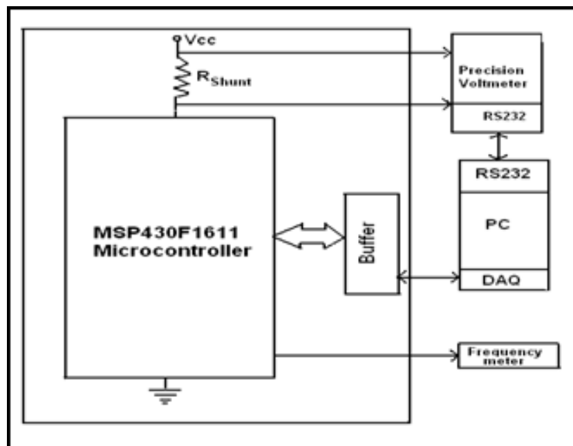
Figure 8. Measurement of current consumption
