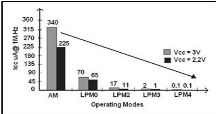
Figure 1. Graph showing the current consumption in different operating modes of MSP430 family.
