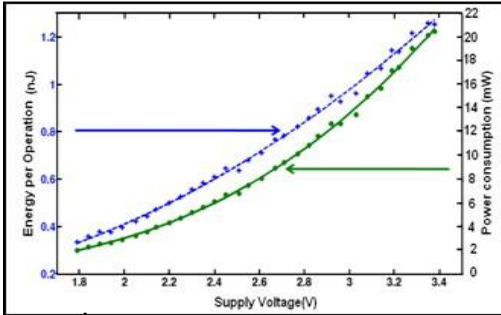
Figure 9. Energy and Power consumption with supply voltage in a MSP430 microcontroller
