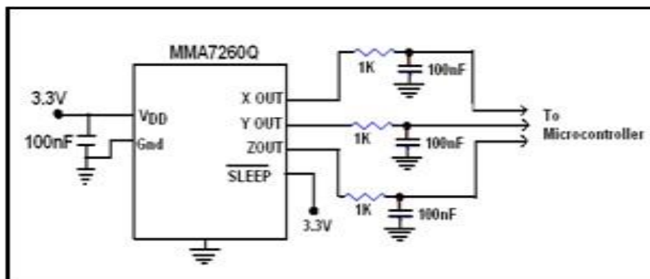
Figure 6. Accelerometer Circuit for respiration measurement
