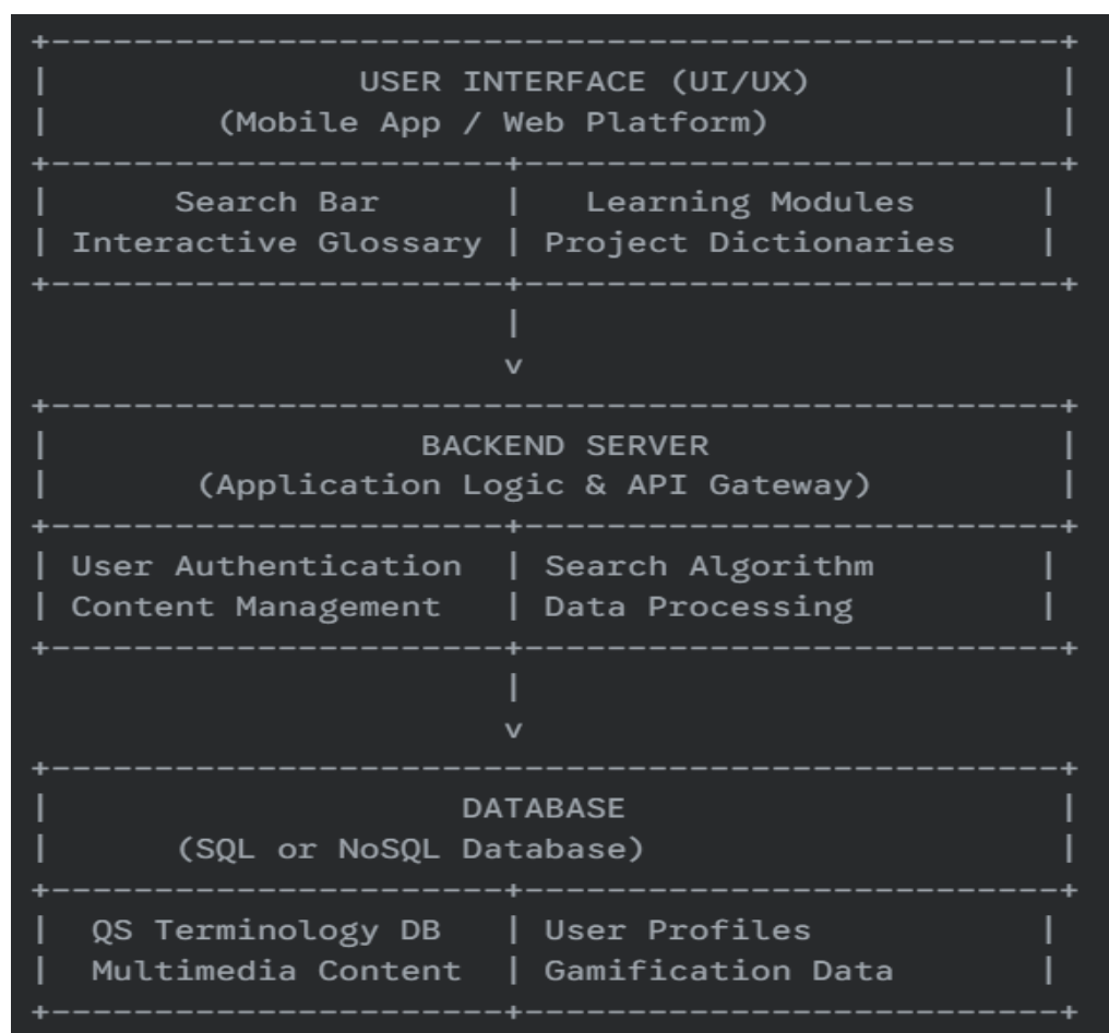
Figure 2: Proposed System Architecture for QS Jargon Apps
