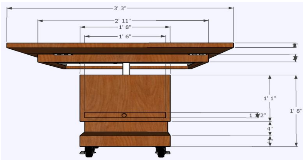
Figure 5 shows the Left Side View of the Ergonomic Garment Table with Hydraulic Height Adjustment Mechanism with Parts
