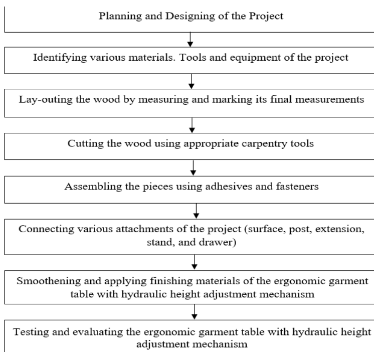
Figure 9: Workflow of the construction of the ergonomic garment table with a hydraulic height adjustment mechanism
