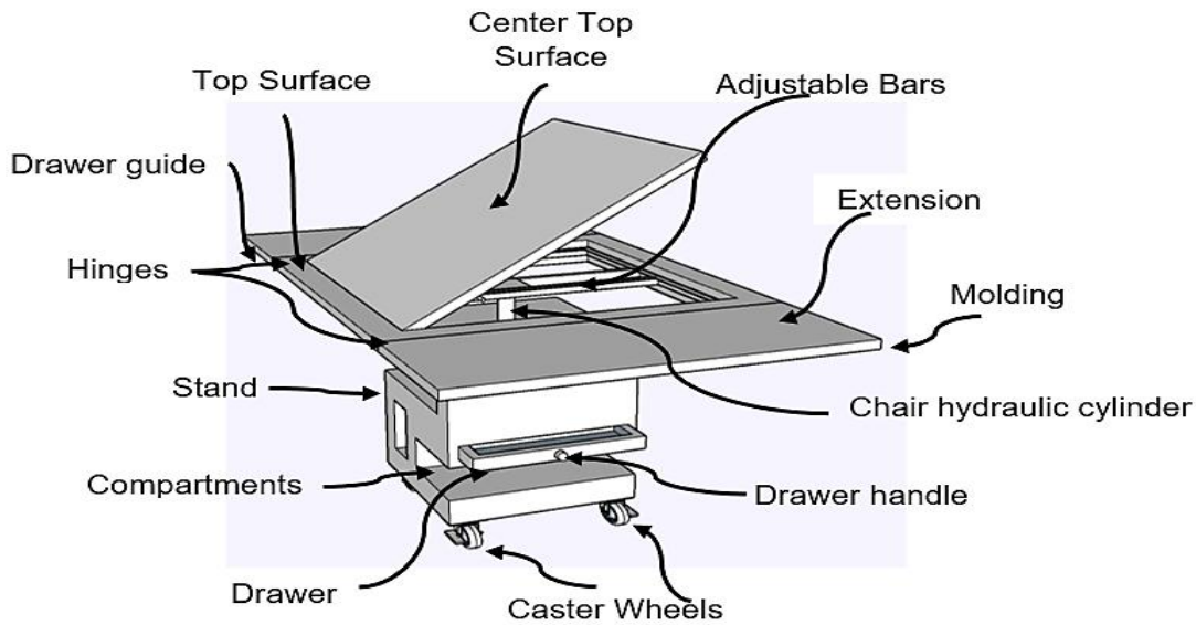
Figure 2: Pictorial Drawing of the Ergonomic Garment Table with Hydraulic Height Adjustment Mechanism with Parts
