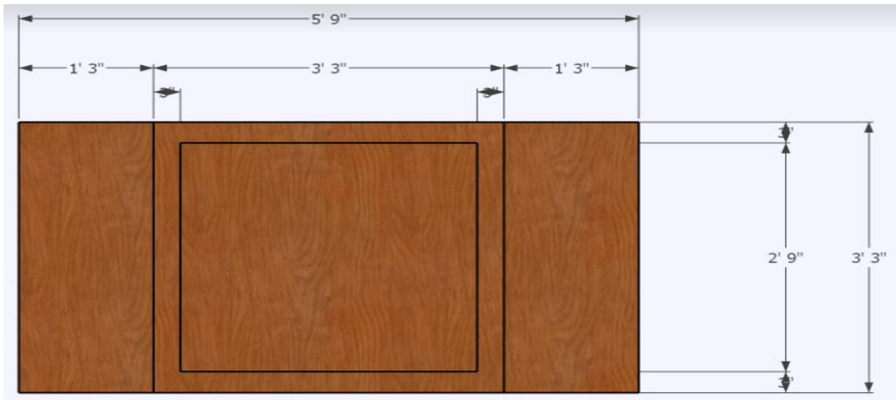
Figure 3 shows the Top View of the Ergonomic Garment Table with Hydraulic Height Adjustment Mechanism with Parts
