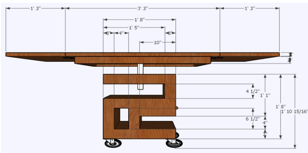
Figure 6 shows the Front View of the Ergonomic Garment Table with Hydraulic Height Adjustment Mechanism with Parts
