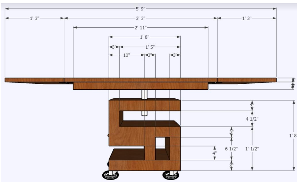
Figure 6 shows the Front View of the Ergonomic Garment Table with Hydraulic Height Adjustment Mechanism with Parts
