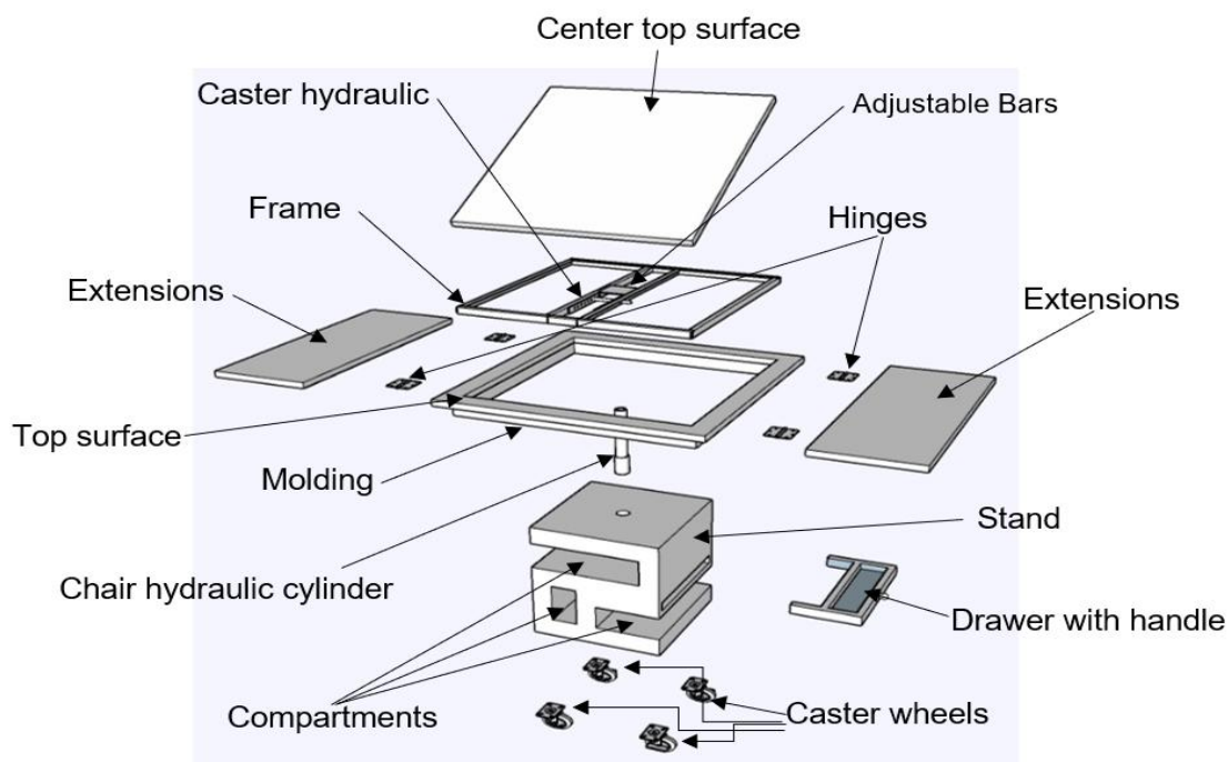
Figure 8: Exploded Drawing of the Ergonomic Garment Table with Hydraulic Height Adjustment Mechanism with Parts
