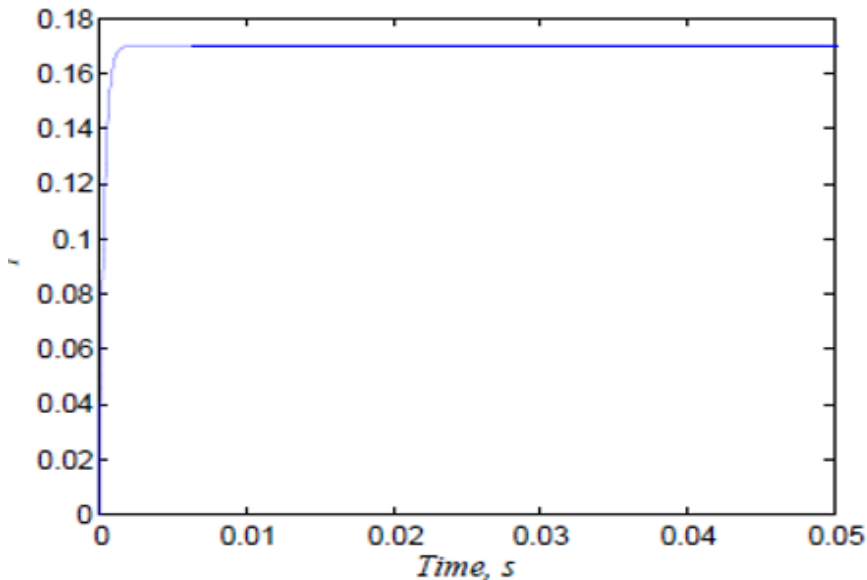
Figure 3: Inner approximation for x
