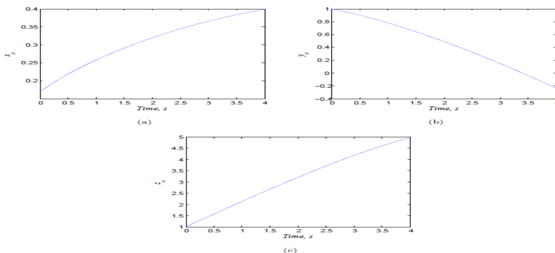
Figure 2: Outer approximations of x , y and z
