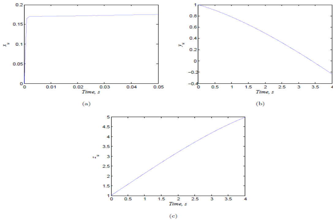
Figure 4: Uniform approximations of x , y and z
