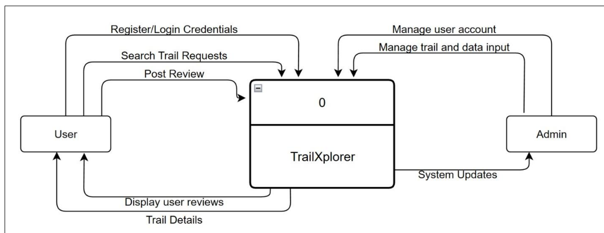
Fig. 3 Context Diagram
