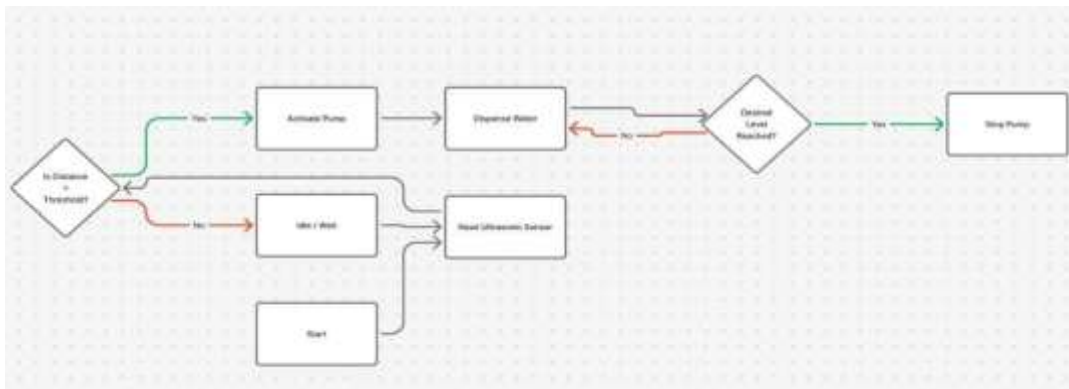
Figure 7. Flow Chart
