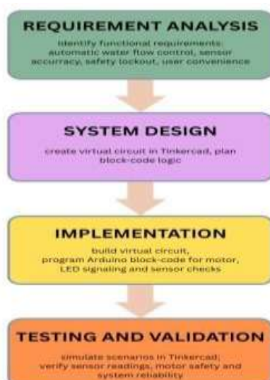
Figure 6. Waterfall Model
