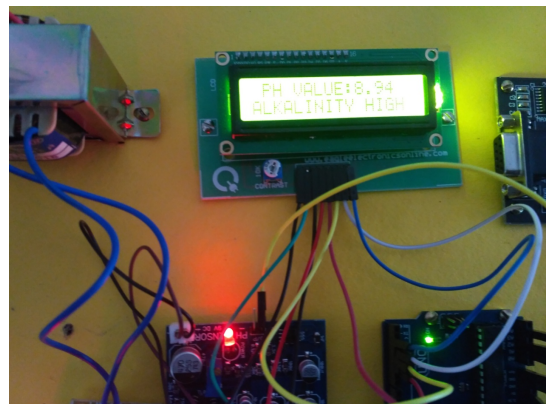
Figure.7. Added alkalinity level of water output
