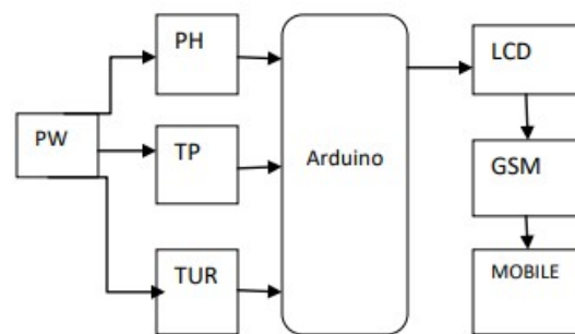
Fig1: Block diagram of H 2 O Auto check
