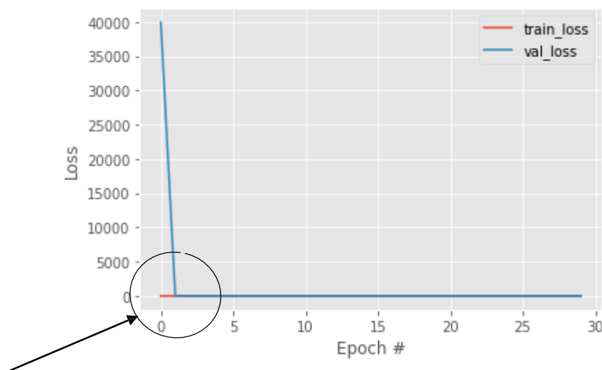
Figure 5: Model Loss
