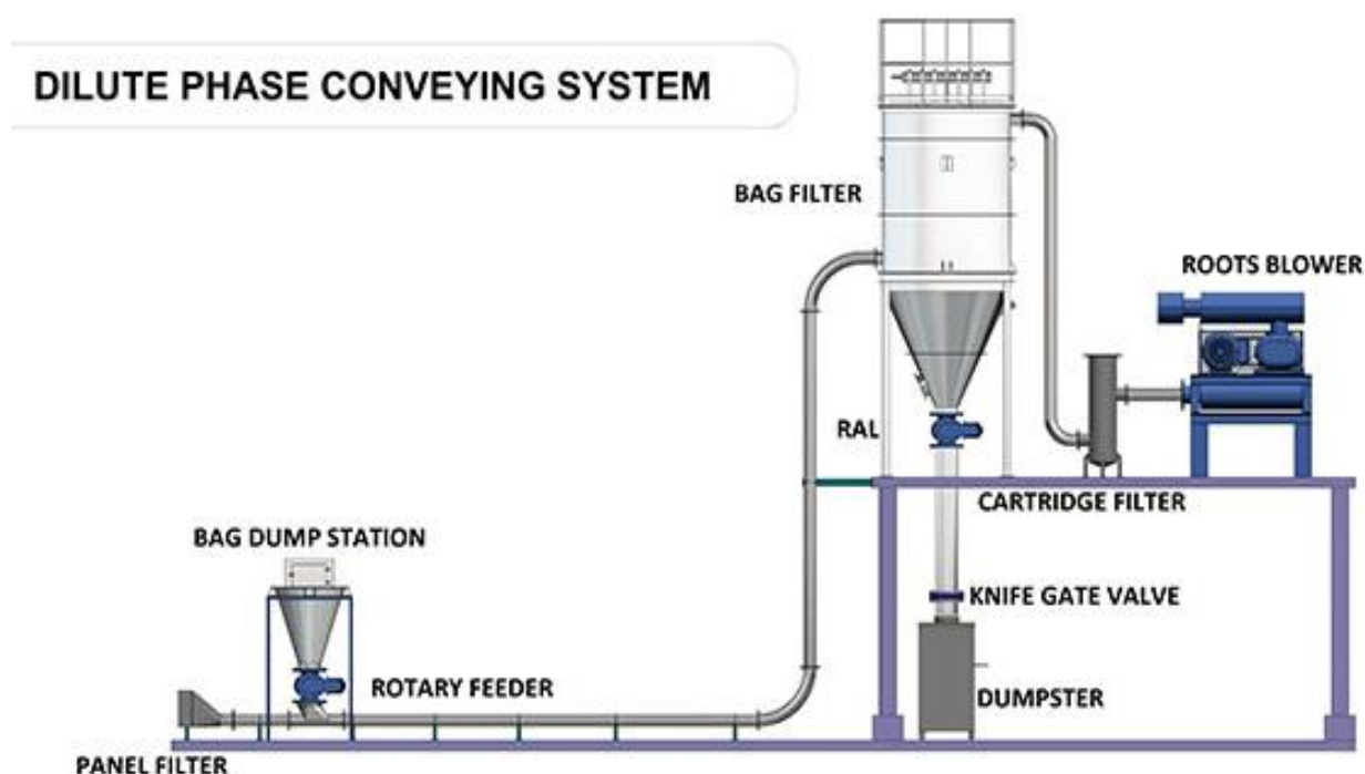
Fig a: Lean Phase System
