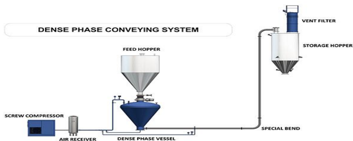
Pic 1b: Dense Phase System
