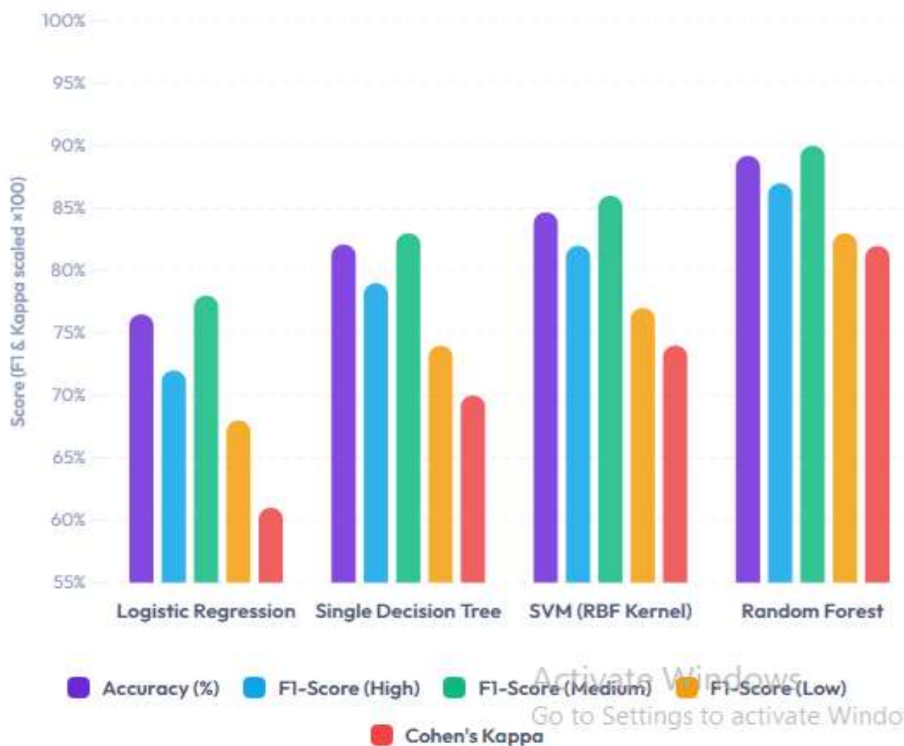
Figure 2. Performance Comparison of Machine Learning Models in AEPAS Framework
