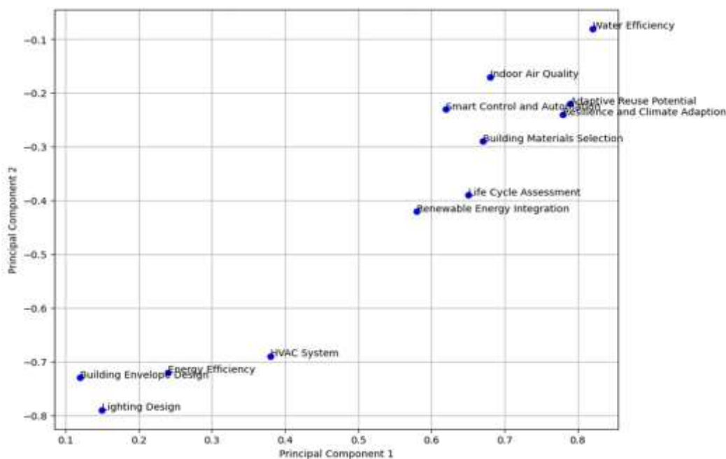
Figure 4. Biplot of the Rotated Principal Components
