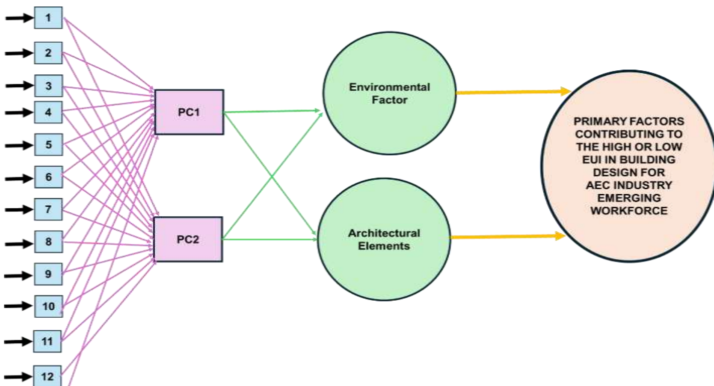
Figure 5. The Study's PCA Schematic Diagram
