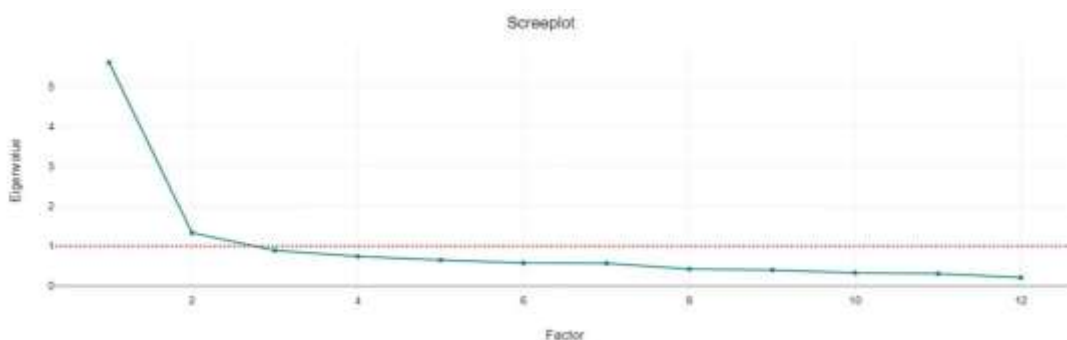
Figure 3. Scree Plot of the PCA Factor Analysis
