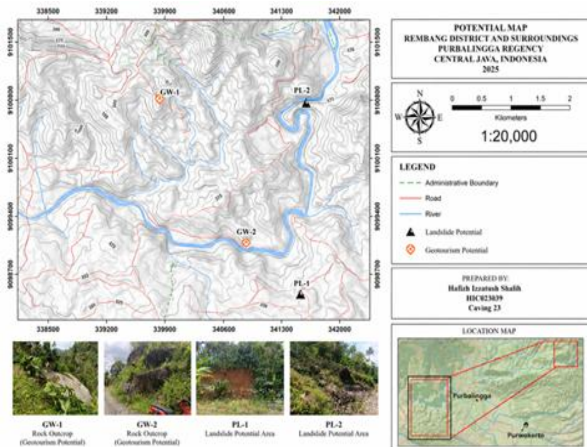
Figure 6. Potential Map Rembang District
