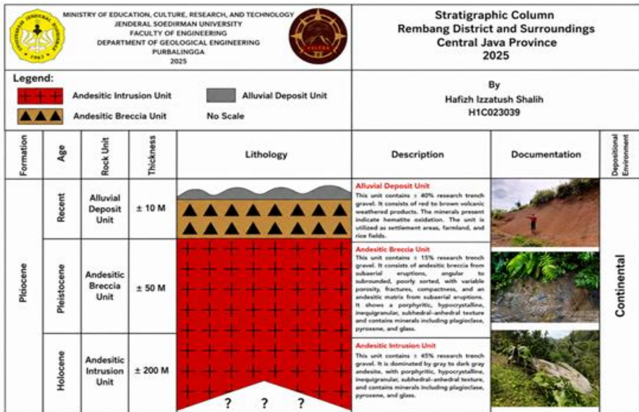
Figure 4. Stratigraphic Column Rembang District and Surrounding Areas, Purbalingga Regency, Central Java, Indonesia
