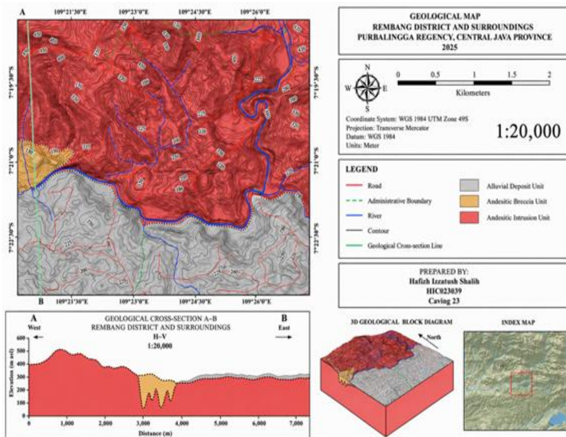
Figure 3. Geological Map of the Rembang District and Surrounding Areas, Purbalingga Regency, Central Java, Indonesia.
