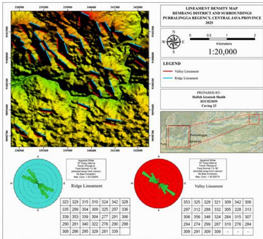
Figure 5. Lineament Density Map Rembang District
